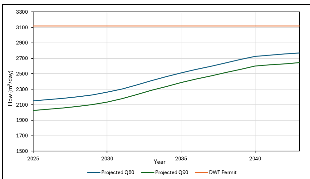
Figure 14 - Immingham WRC Headroom Forecast (2025-2043)
