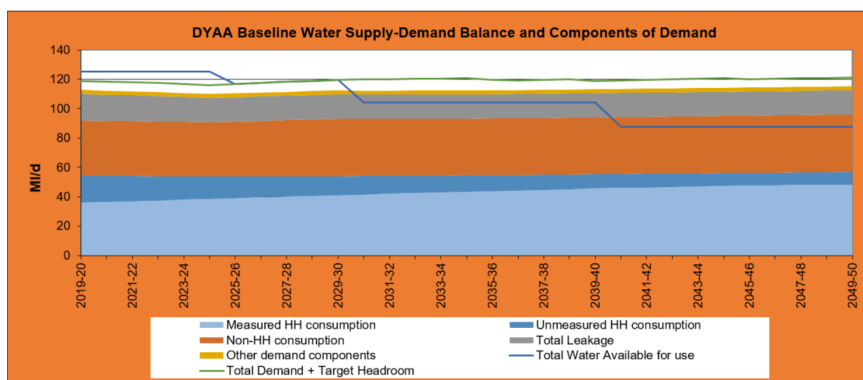
Figure 6 - Baseline Water Supply-Demand Balance (Lincolnshire East WRZ)
