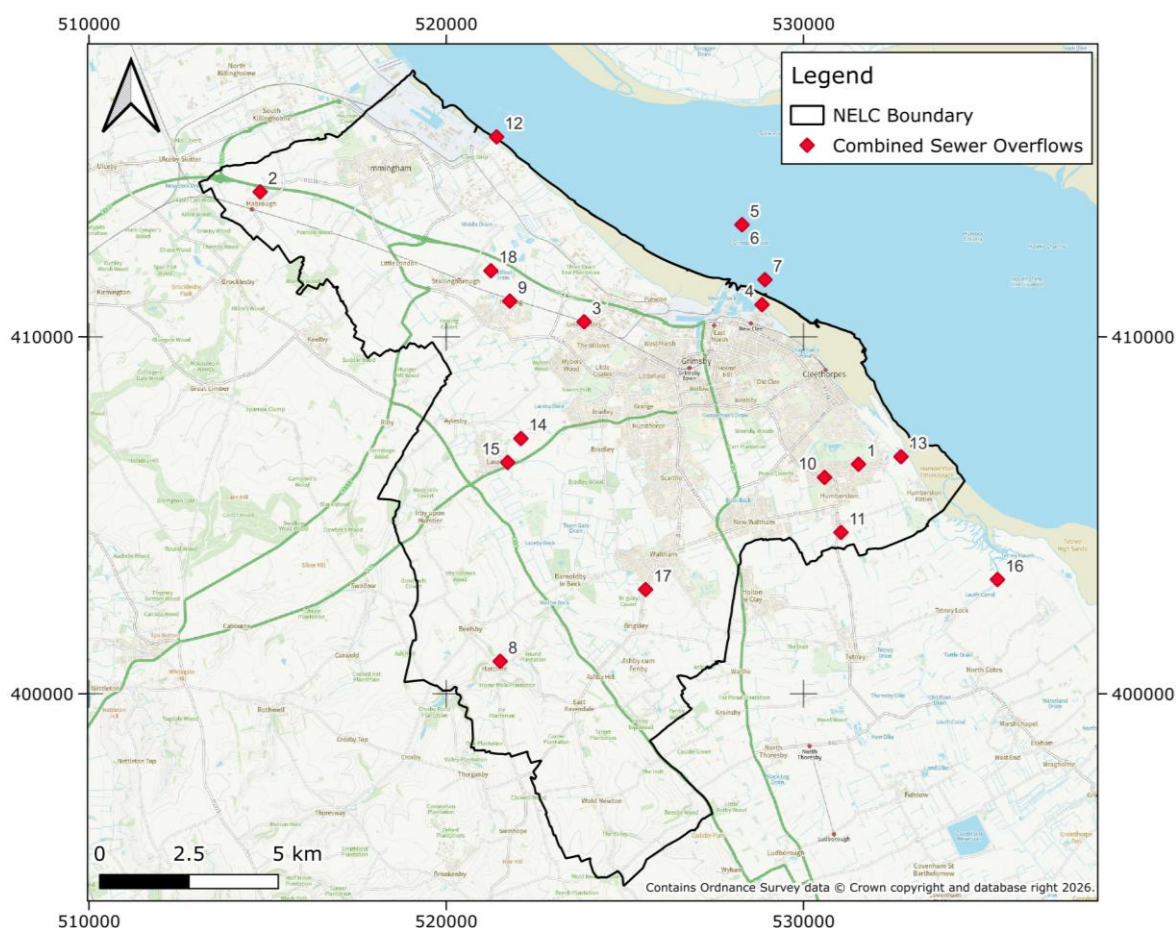
Figure 12 - CSO Discharge Locations
