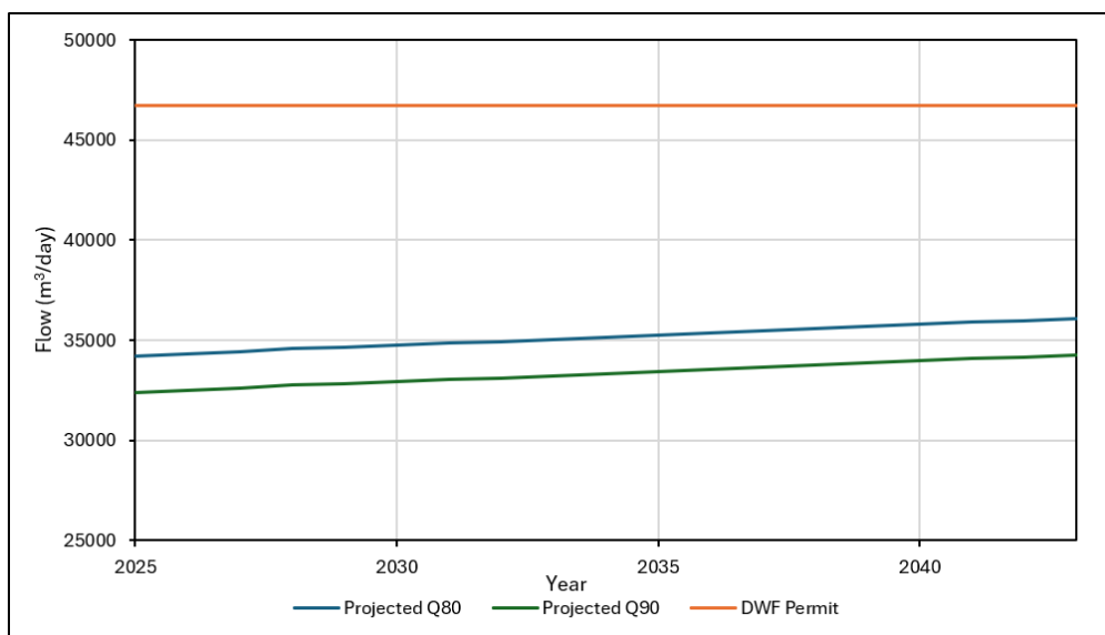
Figure 16 – Grimsby-Pyewipe WRC Headroom Forecast (2025-2043)
