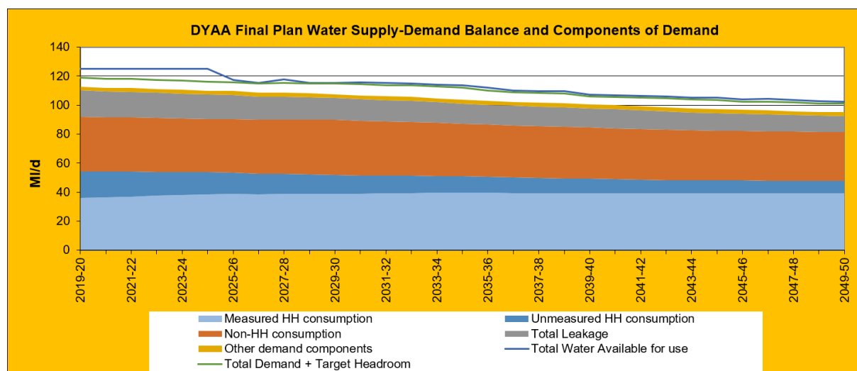
Figure 7 - Final Plan Supply-Demand Balance (Lincolnshire East WRZ)
