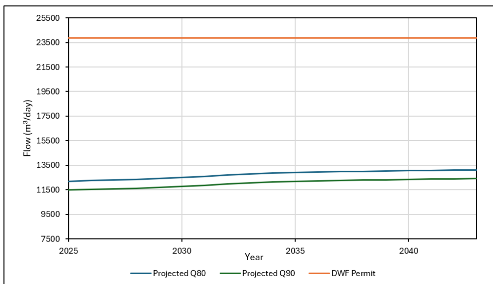
Figure 17 – Tetney-Newton Marsh WRC Headroom Forecast (2025-2043)
