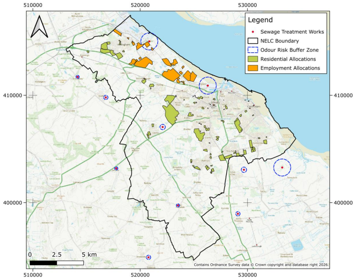
Figure 25 - WRC Odour Risk Buffer Zones
