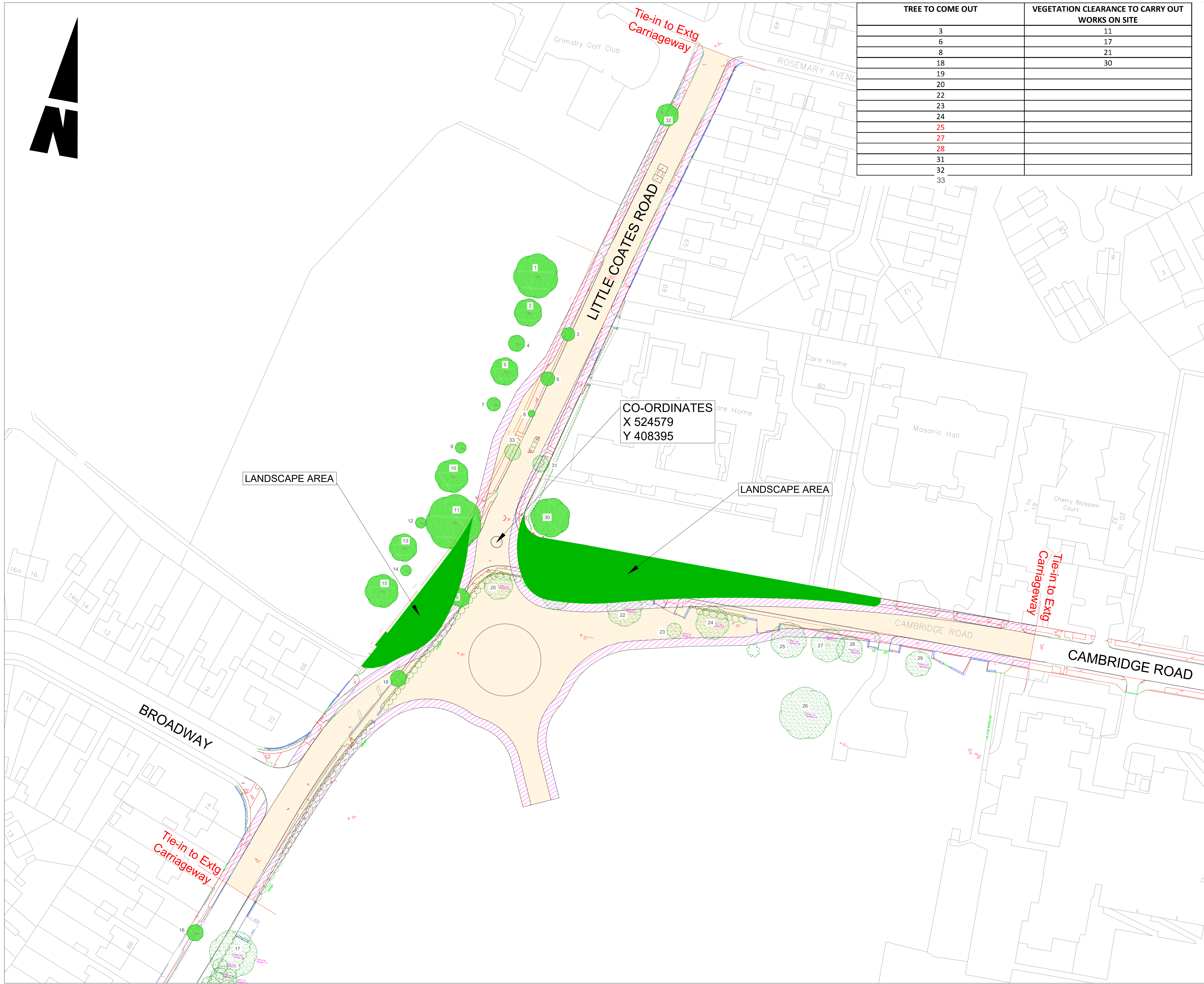
PRELIMINARY ROUNDABOUT (SCALE 1:500)
